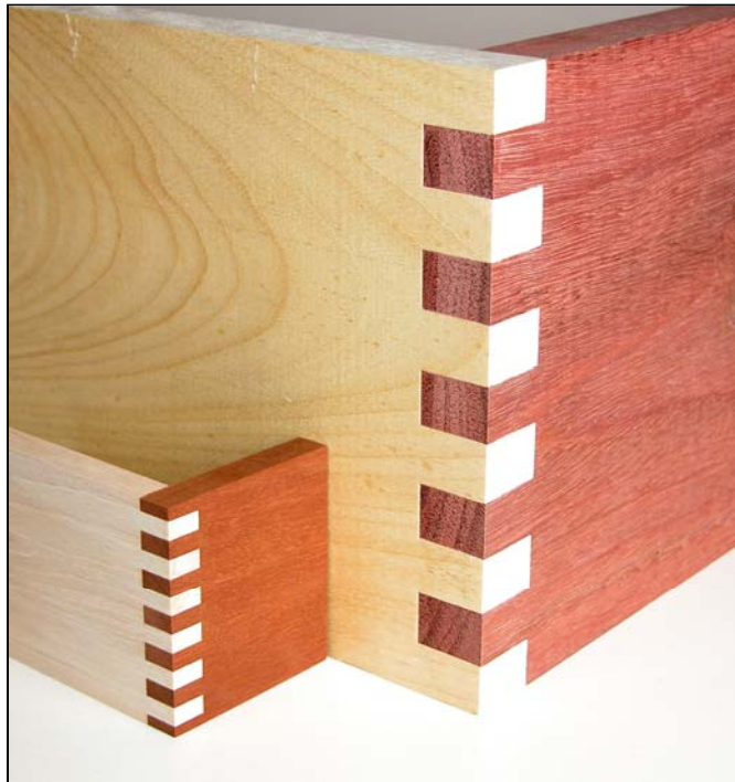
Photo shows F5 joint in 10 mm timber and F15 joint in 20 mm timber
